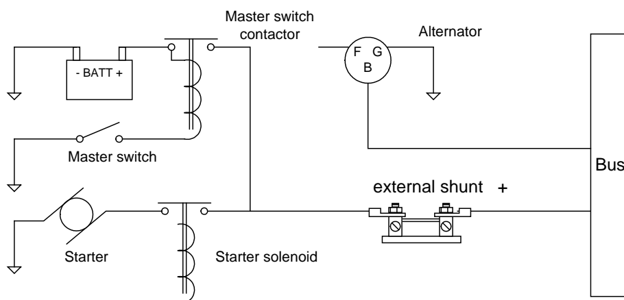
Ammeter Configuration
